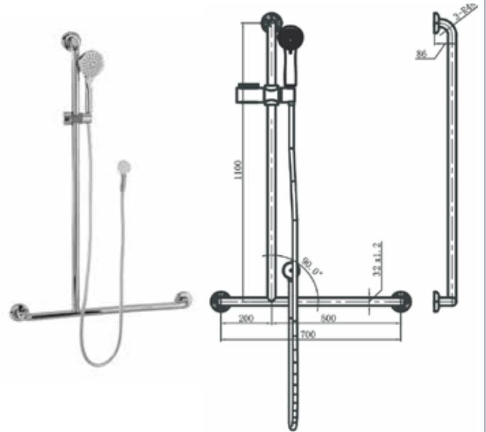
T SHAPED GRAB RAIL SHOWER SET LEFT HAND Compliance with AS1428.1-2021
