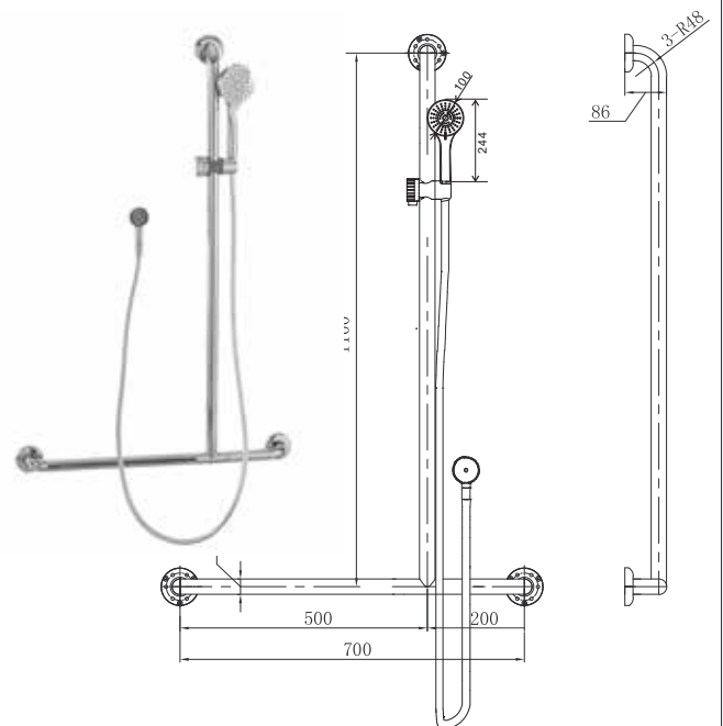
T SHAPED GRAB RAIL SHOWER SET RIGHT HAND Compliance with AS1428.1-2021
