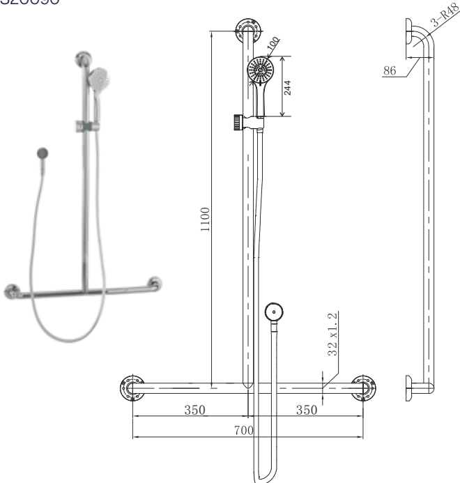
T SHAPED GRAB RAIL SHOWER SET CENTRE Compliance with AS1428.1-2021
